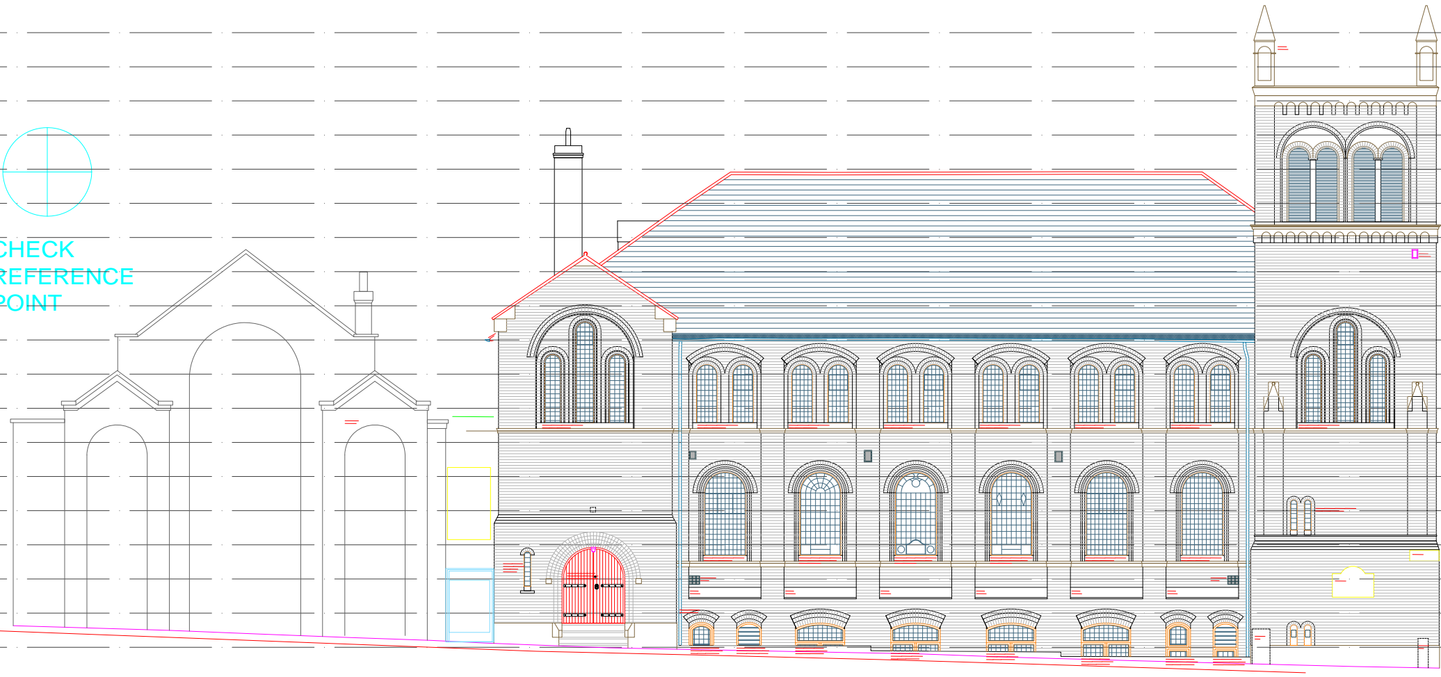
SIDE ELEVATION
